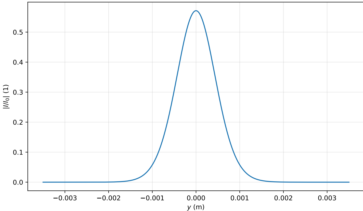
Intensity profile I(x=0, y, z=2.309)/I_0 , P_{in}=0.3P_{cr} , artificial time
